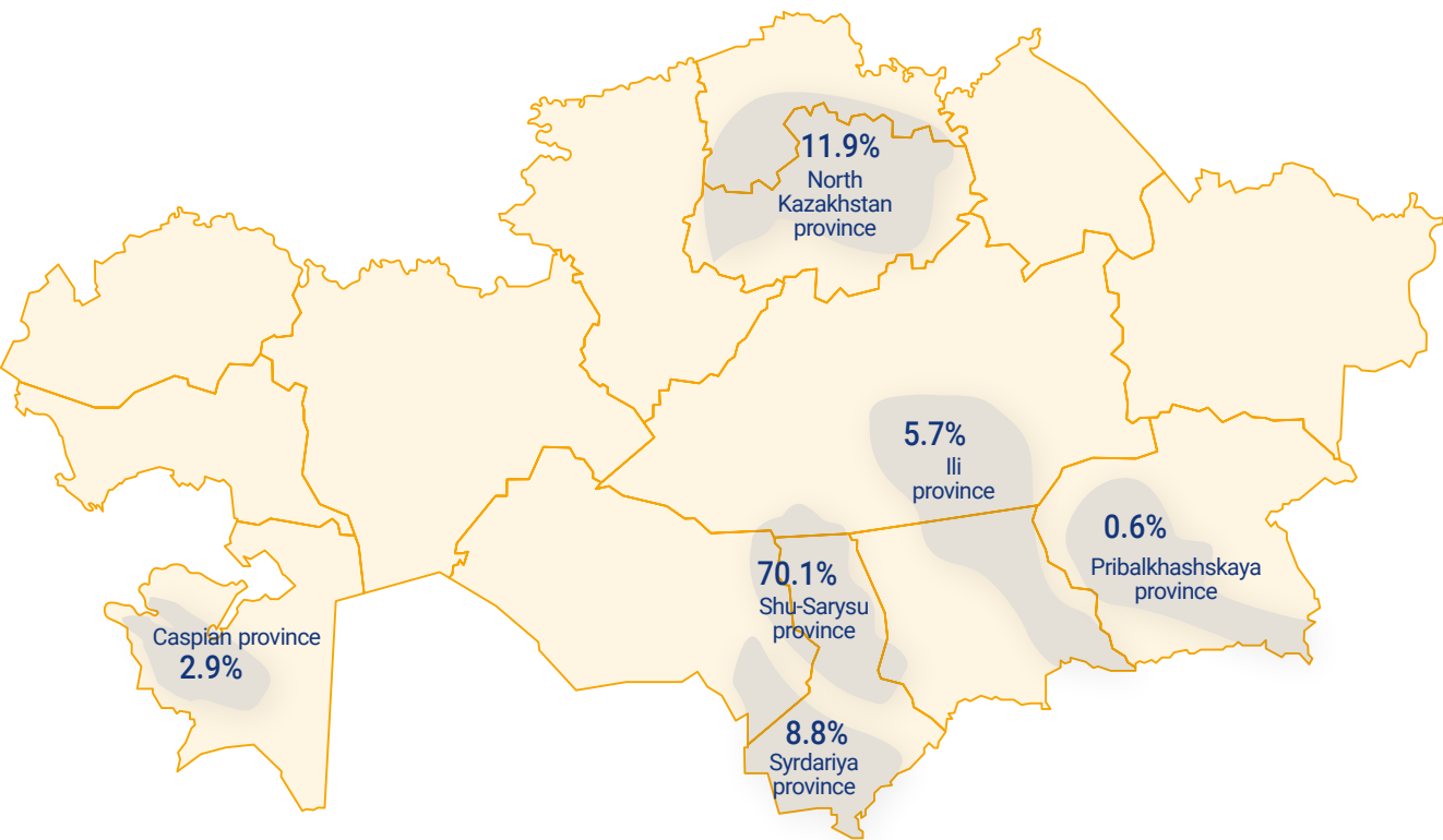
Kazakhstan's uranium provinces and distribution of uranium reserves based on the State Commission on Mineral Reserves standard 3
